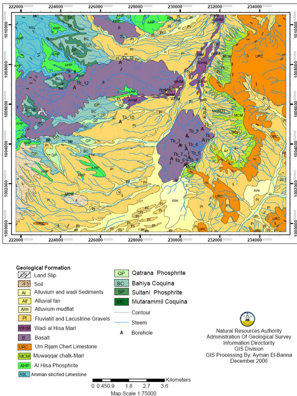
Figure (2): Geological map of Tell Burma area shows boreholes location.
