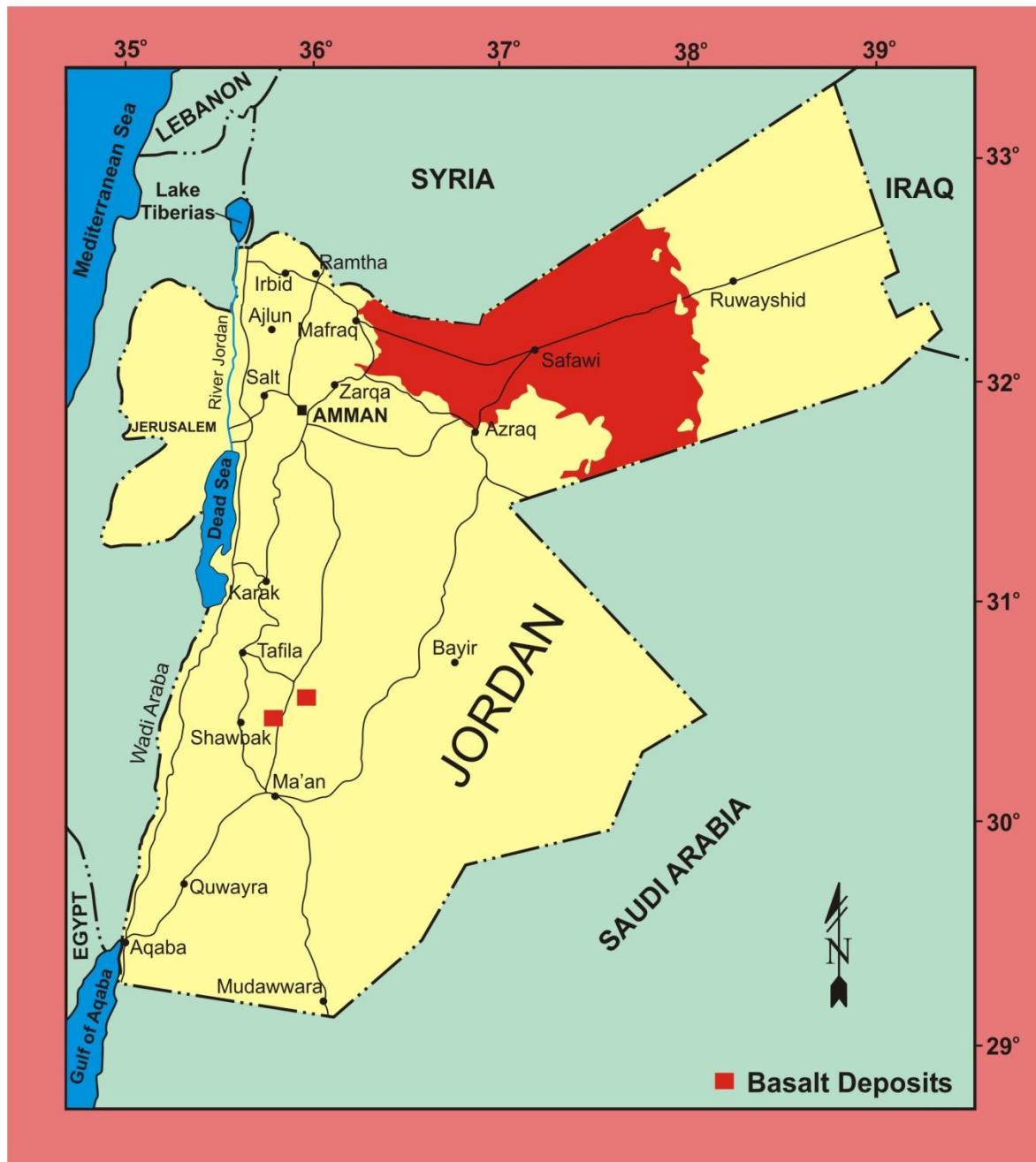
Figure (1): Basalt occurrences in Jordan.
