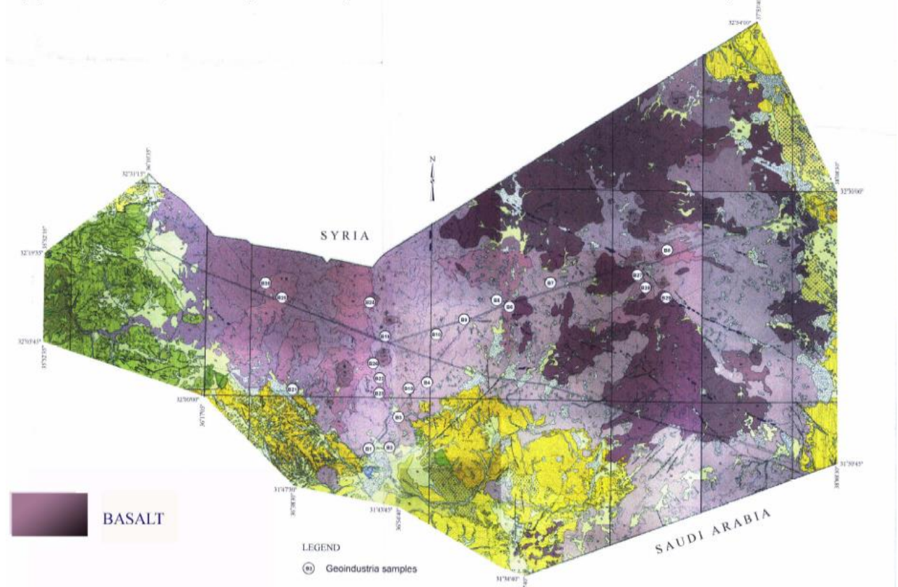
App. (1): Geological map shows plateau Basalt in the north eastern part of Jordan
